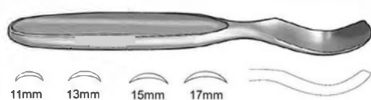
50-498-16 McGlamry Metatarsal Elevator 16 cm / 6 1/2" Sharp
